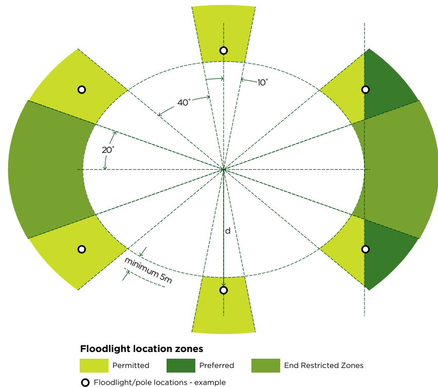
Figure 2: 6 Pole System Source: Adapted figure 3 of IESANZ LG4.01
